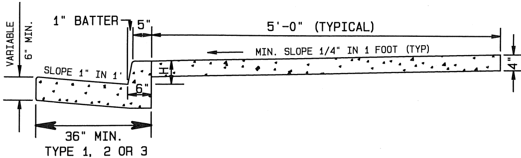
TYPICAL SECTION 36" CURB & GUTTER WITH 4" SIDEWALK
